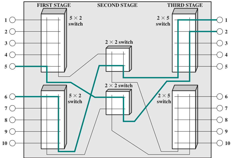
Figure 9.6 Three-Stage Space Division Switch
