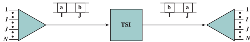
(a) TSI Operation
