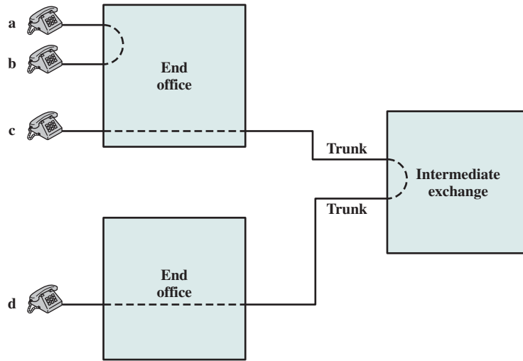
Figure 9.3 Circuit Establishment
